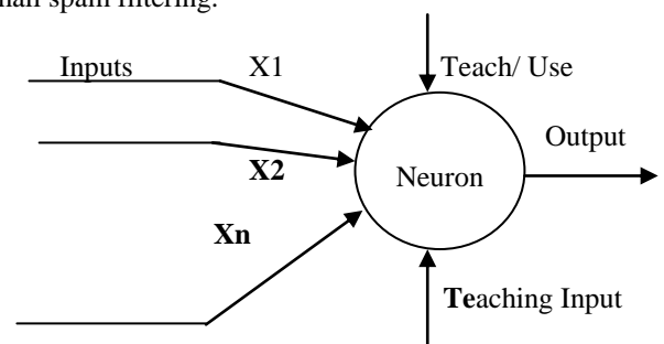
Figure 1 Simple ANN
